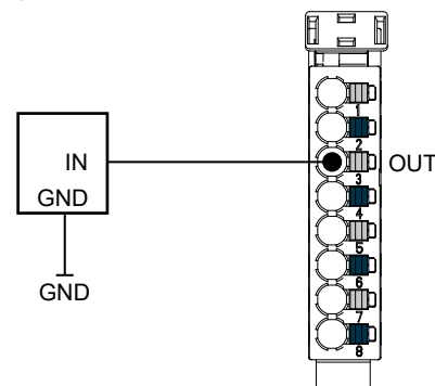
Fig. 2: One-wire actuator
