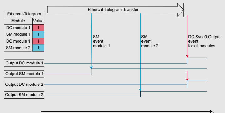
Fig. 1: Temporal response of the outputs for DC- and SM-synchronous modules
