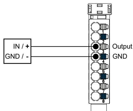
Fig. 3: Two-wire actuator
