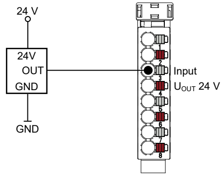
Fig. 2: 1-wire sensor
