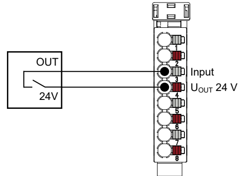
Fig. 3: 1-wire sensor
