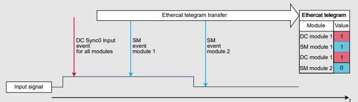
Fig. 1: Temporal response of the reading process for DC- and SM-synchronous modules
