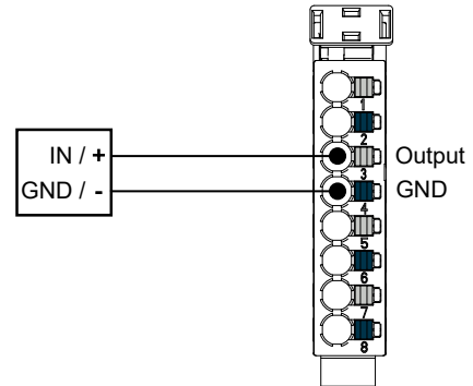
Fig. 4: Two-wire actuator
