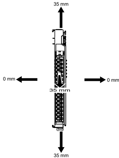
Fig. 5: Ventilation distances
