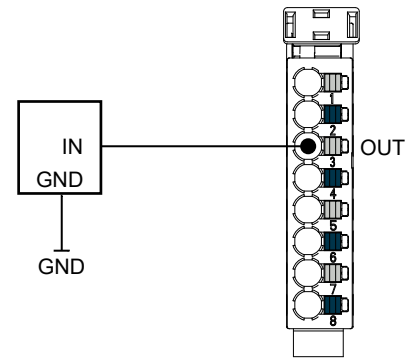
Fig. 3: One-wire actuator
