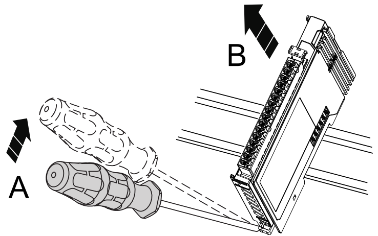
Fig. 9: Removing module from support rail
