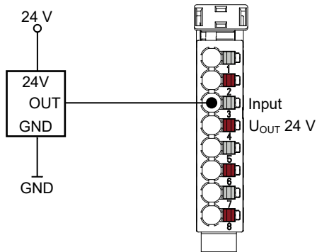
Fig. 3: 1-wire sensor
