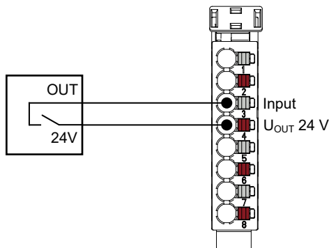
Fig. 4: 1-wire sensor
