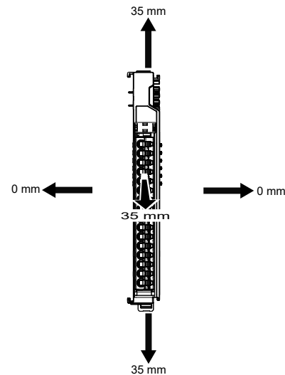
Fig. 5: Ventilation distances
