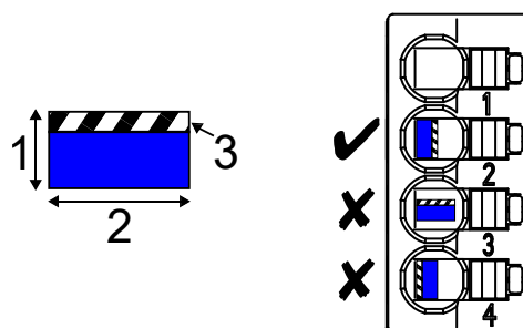
Fig. 11: Orientation of the wire end ferrules in the clamping point
