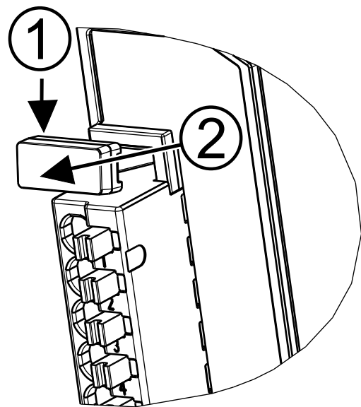
Fig. 8: Removing plug
